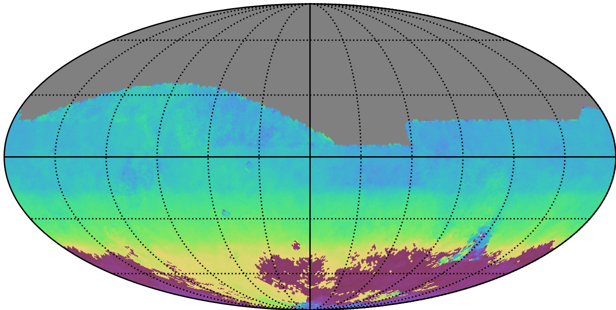
extra_ss_neo4_v3.4_10yrs All sky z band: AngleMean rotSkyPos
