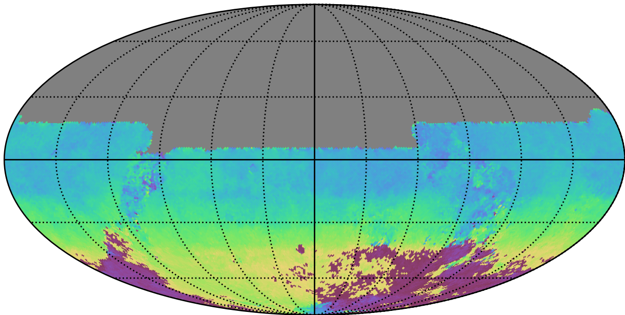
extra_ss_neo4_v3.4_10yrs All sky u band: AngleMean rotSkyPos
