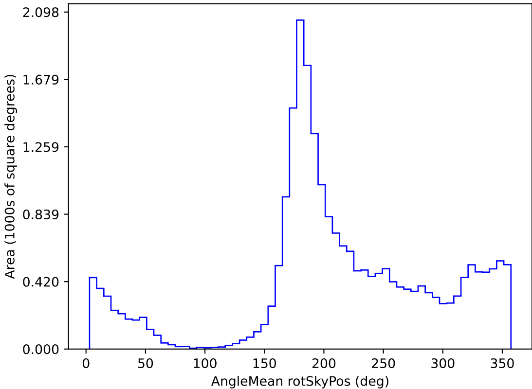
extra_ss_neo4_v3.4_10yrs All sky u band: AngleMean rotSkyPos
