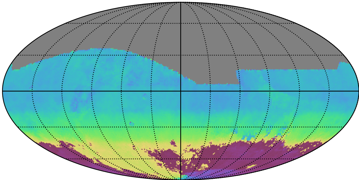
extra_ss_neo4_v3.4_10yrs All sky r band: AngleMean rotSkyPos
