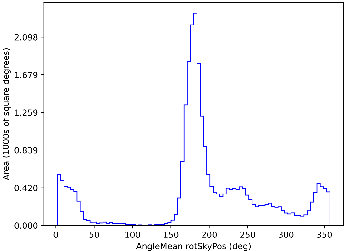
extra_ss_neo4_v3.4_10yrs All sky r band: AngleMean rotSkyPos
