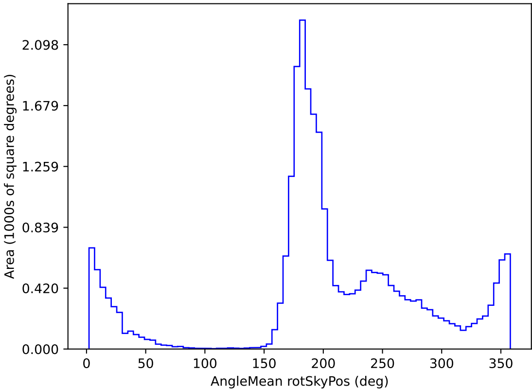
extra_ss_neo4_v3.4_10yrs All sky i band: AngleMean rotSkyPos
