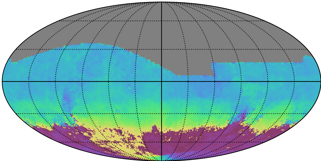
extra_ss_neo4_v3.4_10yrs All sky g band: AngleMean rotSkyPos
