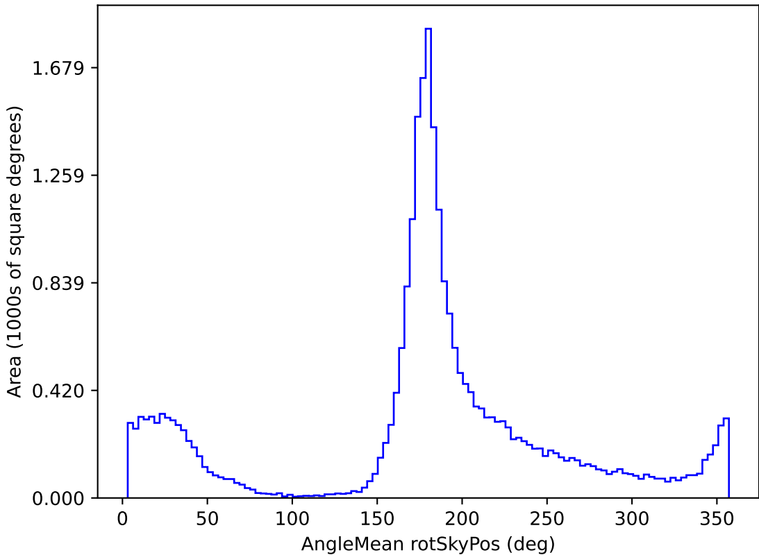
extra_ss_neo4_v3.4_10yrs All sky g band: AngleMean rotSkyPos
