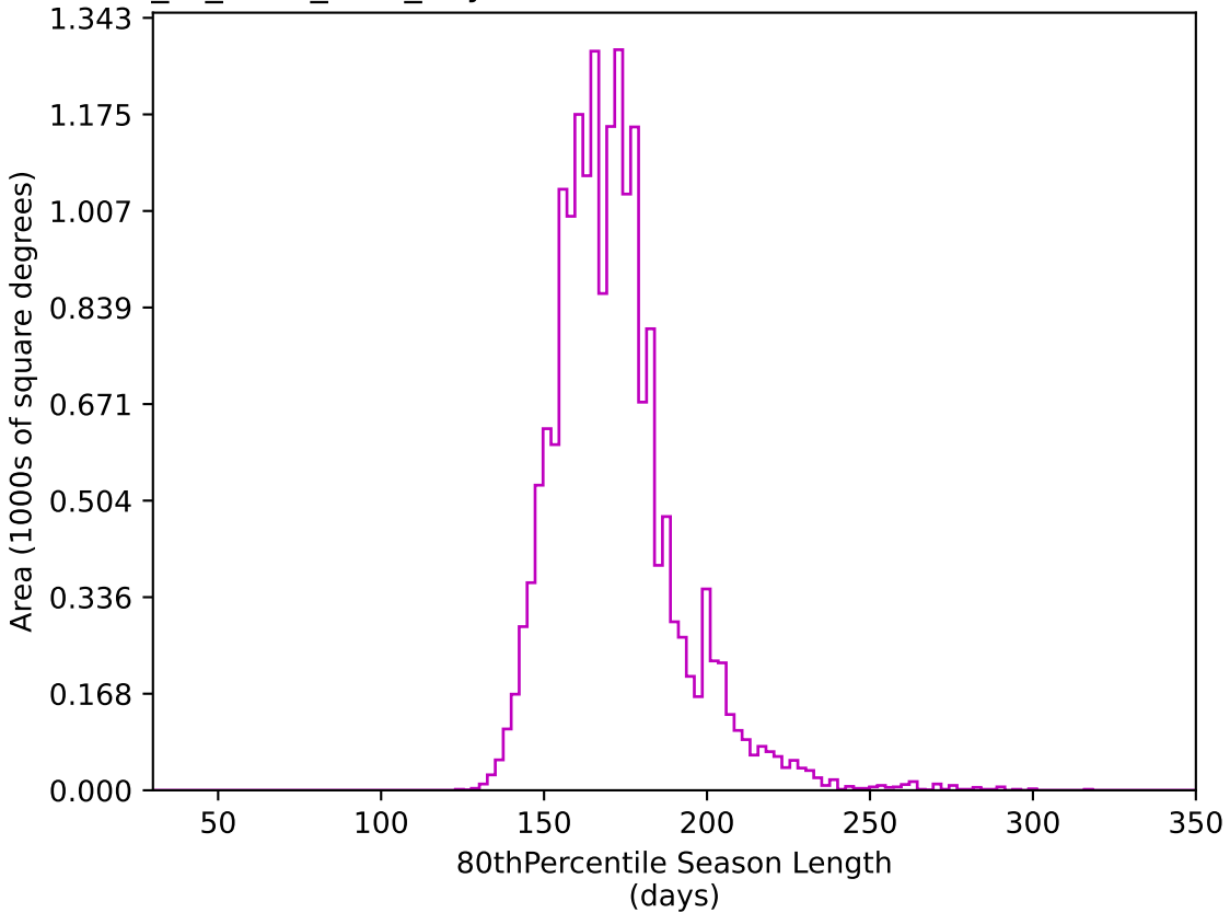
extra_ss_neo4_v3.4_10yrs WFD z band: 80thPercentile Season Length
