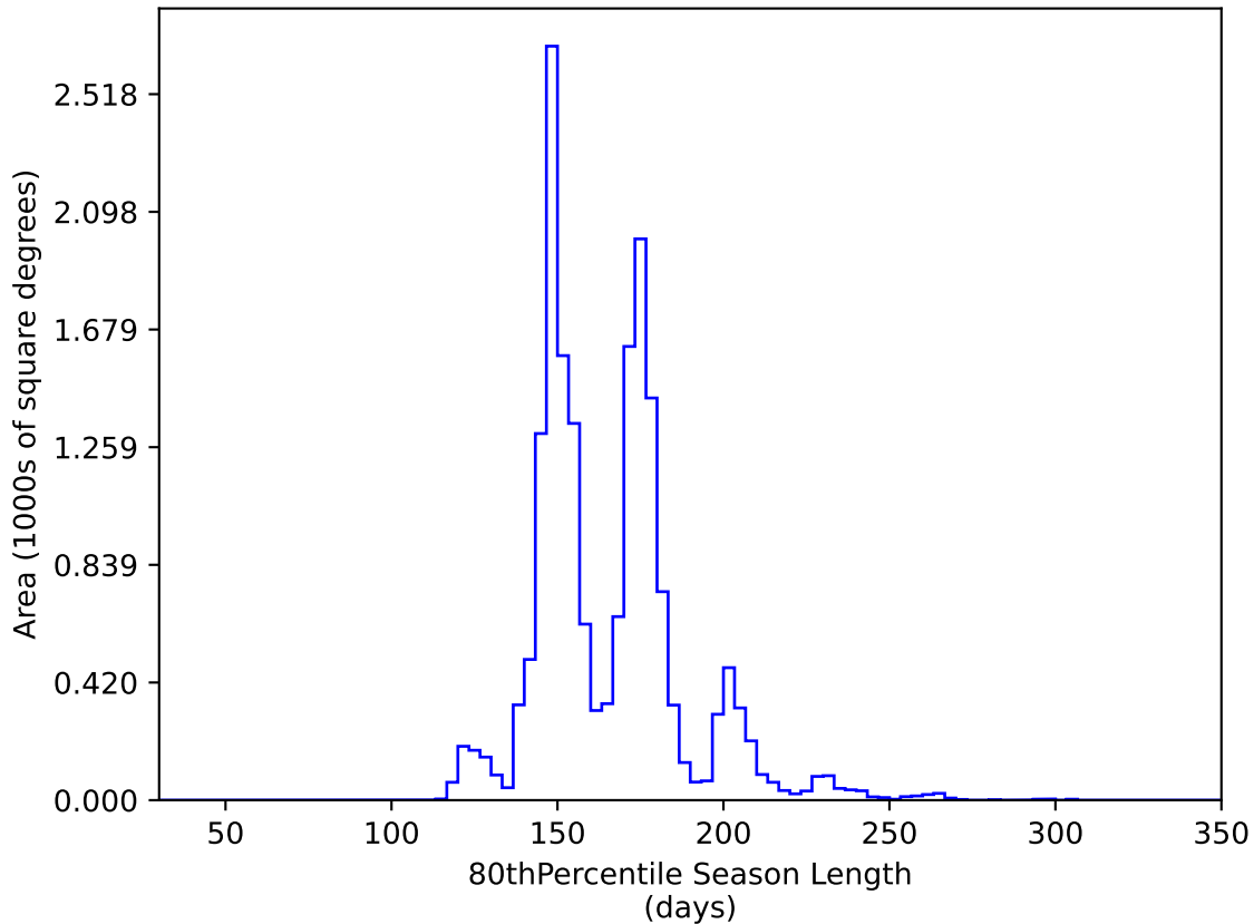
extra_ss_neo4_v3.4_10yrs WFD y band: 80thPercentile Season Length
