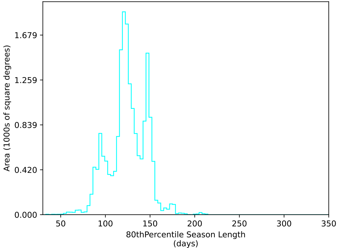
extra_ss_neo4_v3.4_10yrs WFD u band: 80thPercentile Season Length
