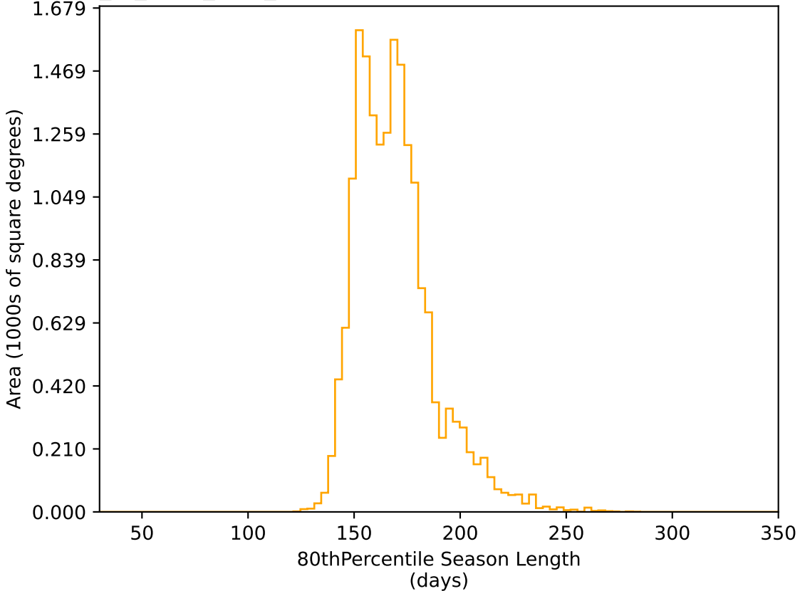
extra_ss_neo4_v3.4_10yrs WFD r band: 80thPercentile Season Length
