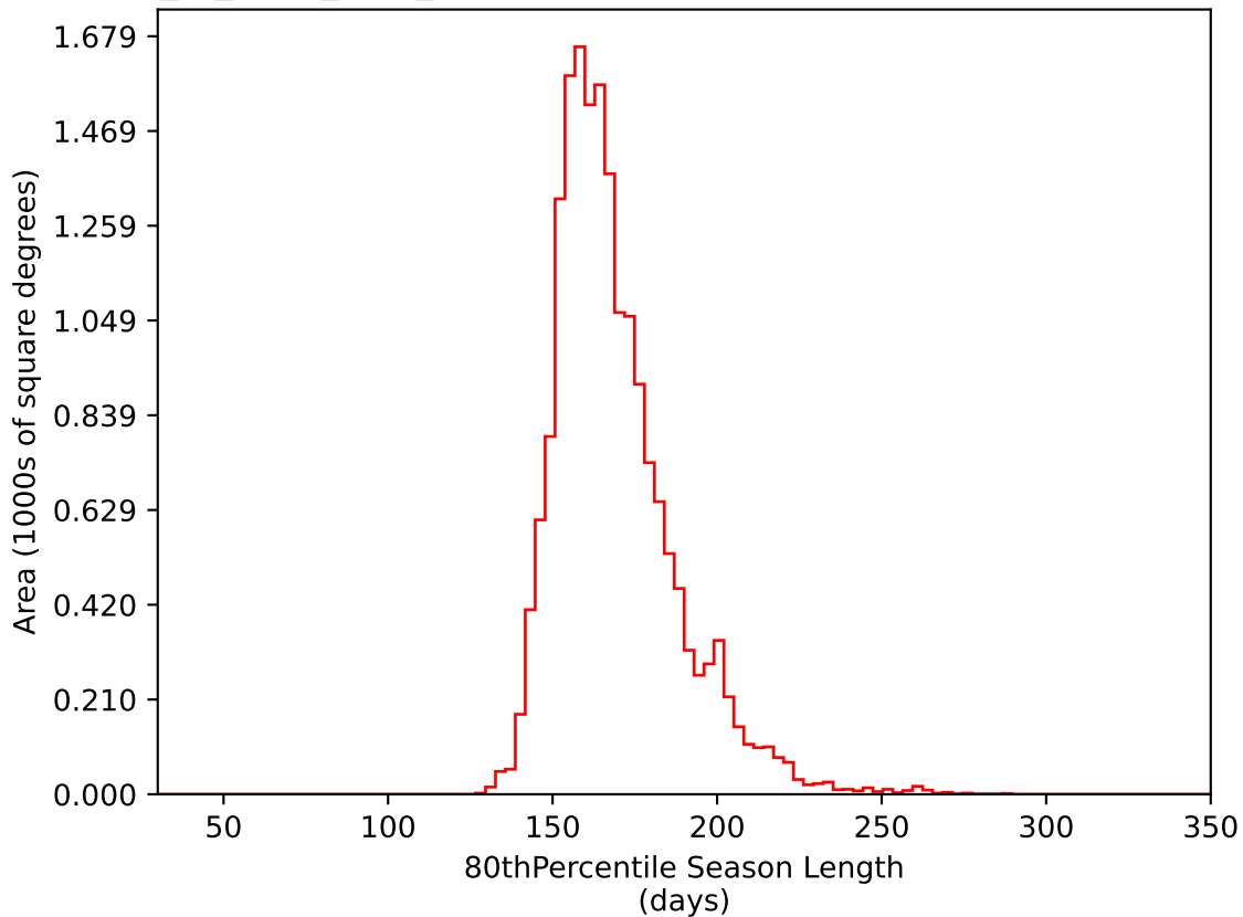
extra_ss_neo4_v3.4_10yrs WFD i band: 80thPercentile Season Length
