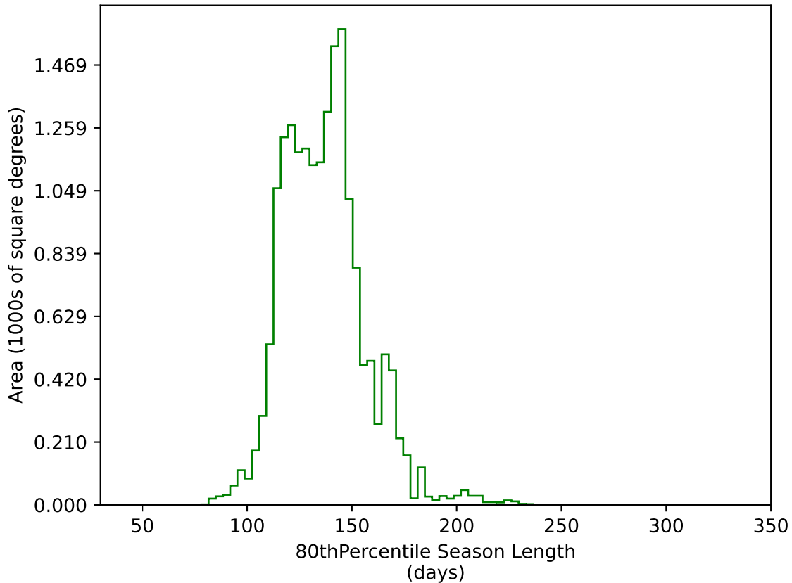
extra_ss_neo4_v3.4_10yrs WFD g band: 80thPercentile Season Length
