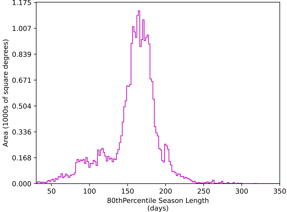
extra_ss_neo4_v3.4_10yrs All sky z band: 80thPercentile Season Length
