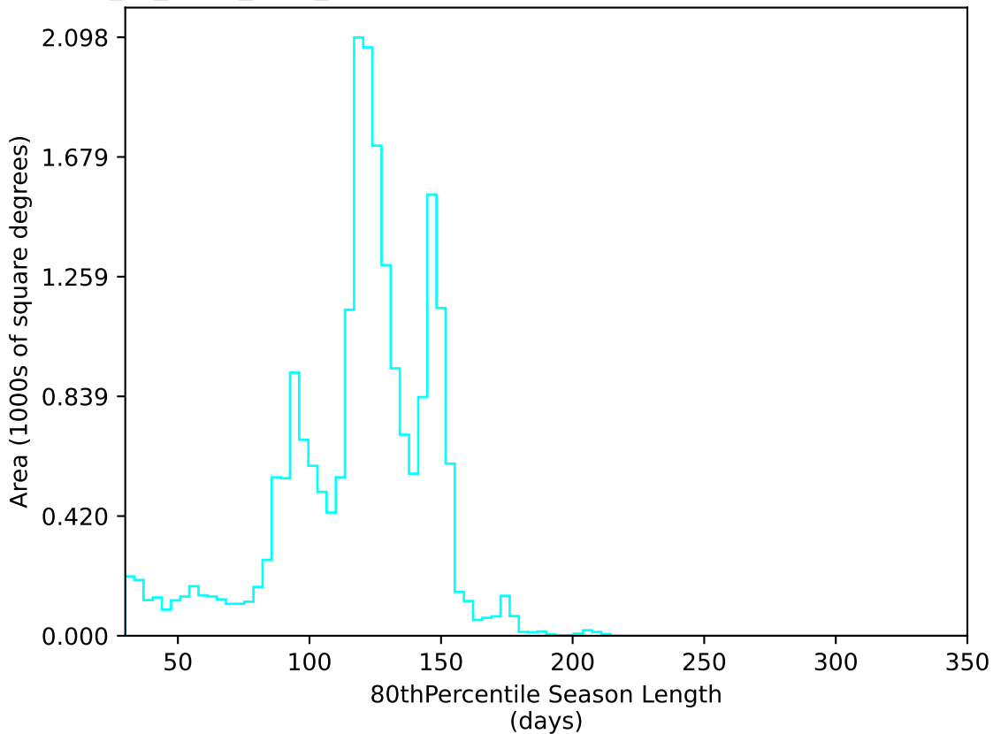
extra_ss_neo4_v3.4_10yrs All sky u band: 80thPercentile Season Length
