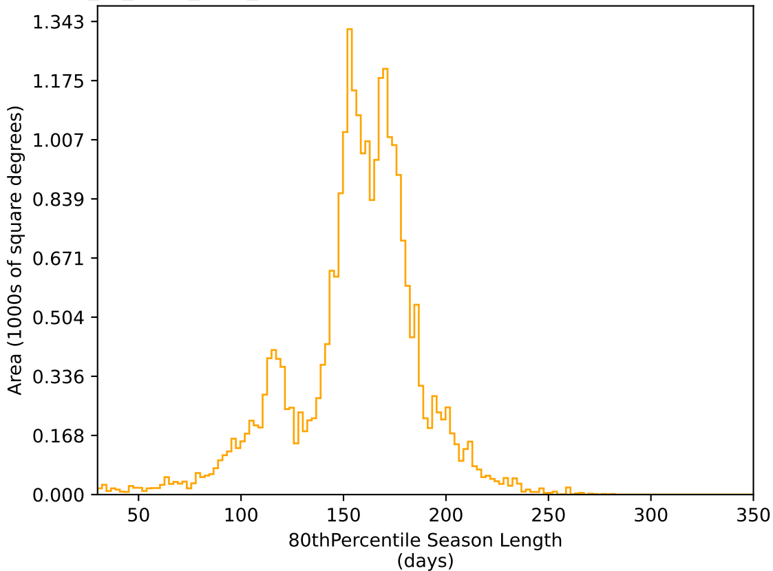
extra_ss_neo4_v3.4_10yrs All sky r band: 80thPercentile Season Length
