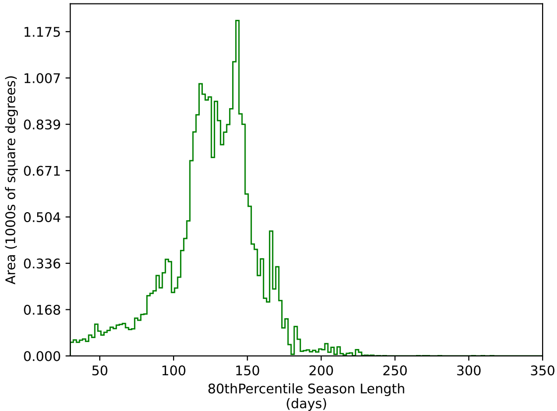
extra_ss_neo4_v3.4_10yrs All sky g band: 80thPercentile Season Length
