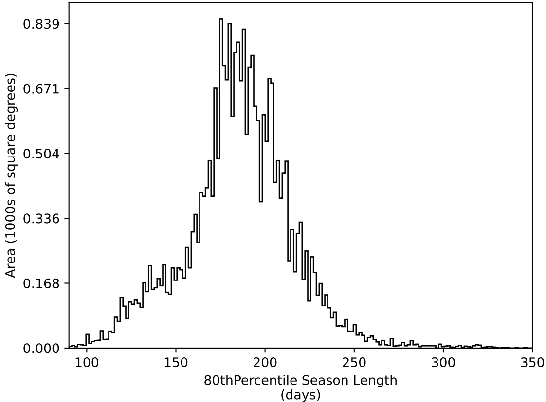
extra_ss_neo4_v3.4_10yrs All sky all bands: 80thPercentile Season Length
