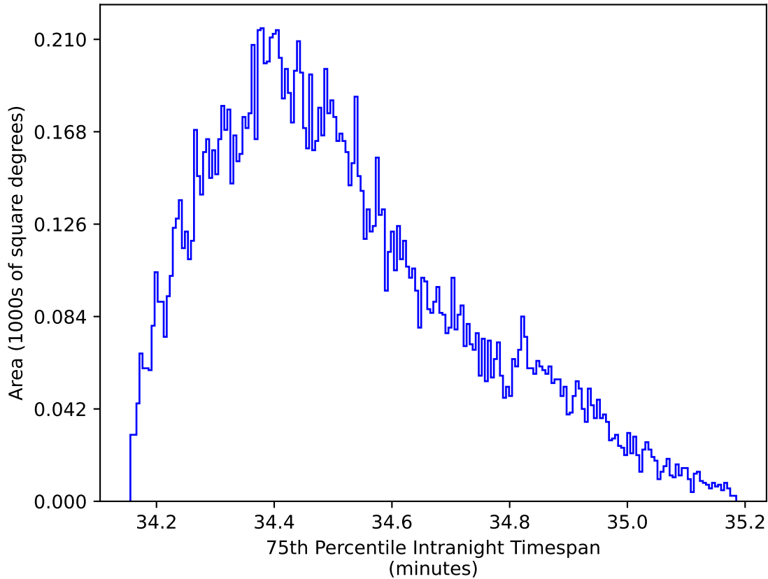
extra_ss_neo4_v3.4_10yrs WFD zy bands: 75th Percentile Intranight Timespan
