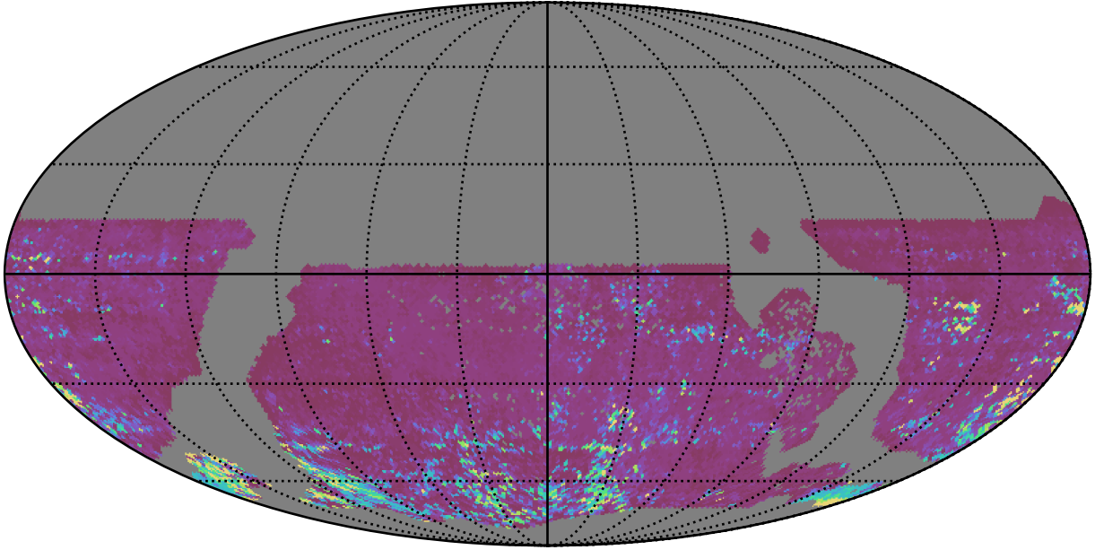
extra_ss_neo4_v3.4_10yrs WFD z band: 75th Percentile Intranight Timespan
