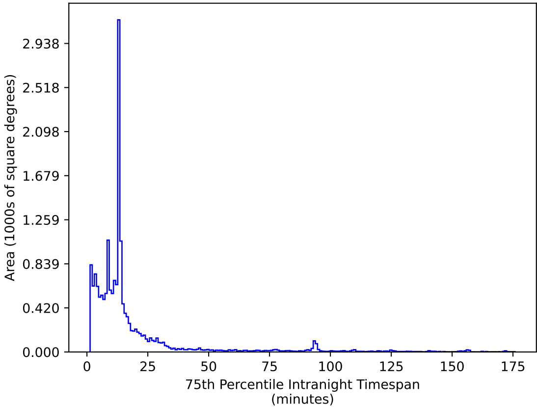
extra_ss_neo4_v3.4_10yrs WFD z band: 75th Percentile Intranight Timespan
