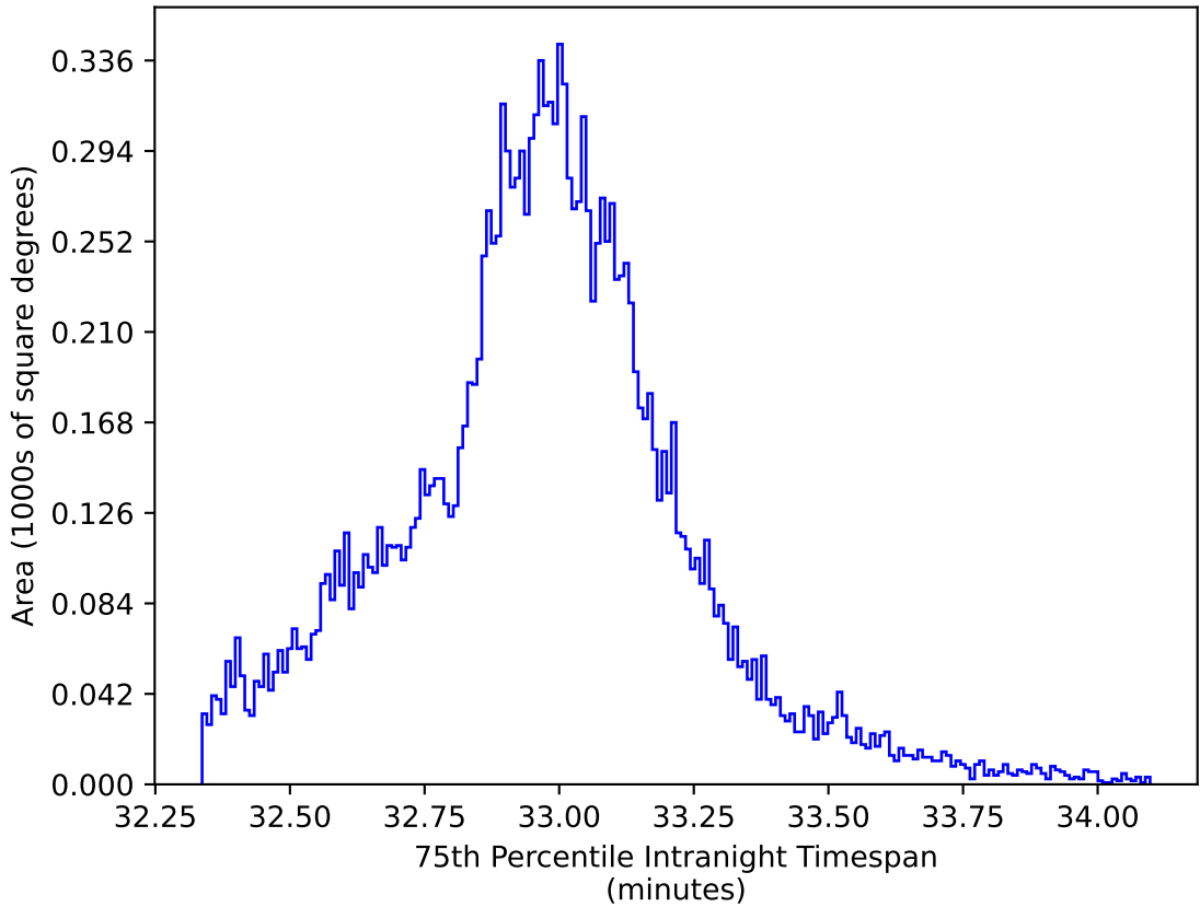
extra_ss_neo4_v3.4_10yrs WFD y band: 75th Percentile Intranight Timespan
