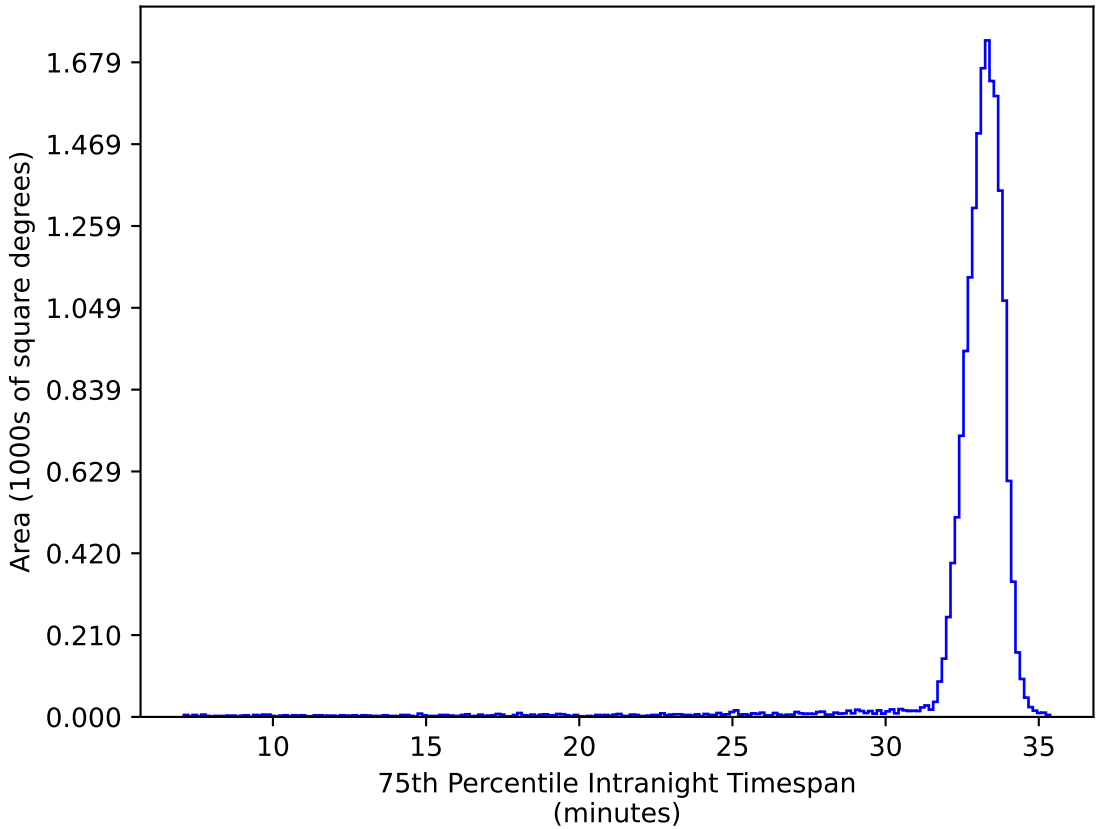
extra_ss_neo4_v3.4_10yrs WFD ug bands: 75th Percentile Intranight Timespan
