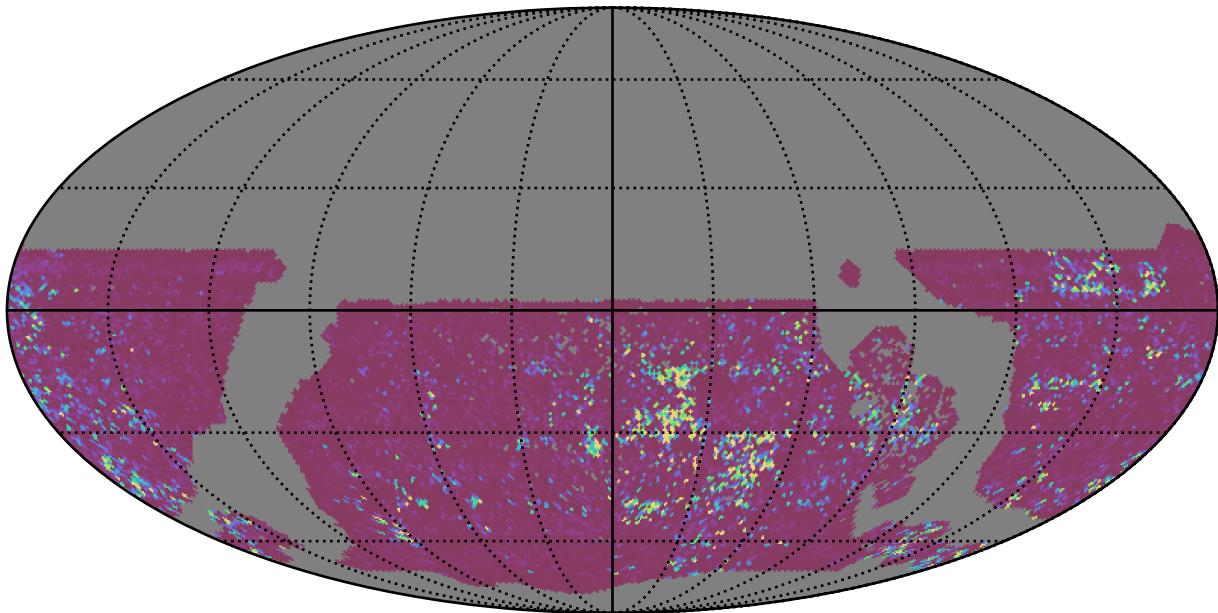
extra_ss_neo4_v3.4_10yrs WFD u band: 75th Percentile Intranight Timespan
