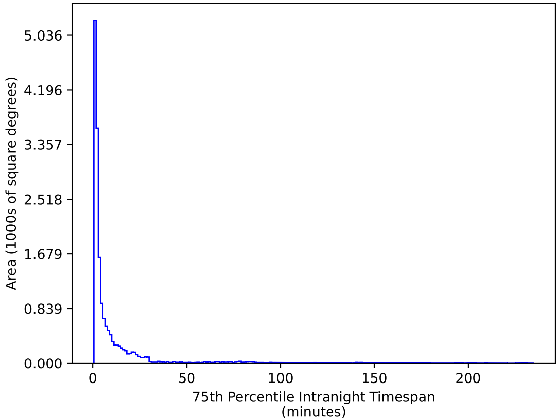
extra_ss_neo4_v3.4_10yrs WFD u band: 75th Percentile Intranight Timespan
