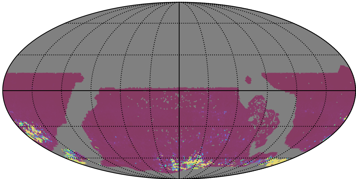
extra_ss_neo4_v3.4_10yrs WFD ri bands: 75th Percentile Intranight Timespan
