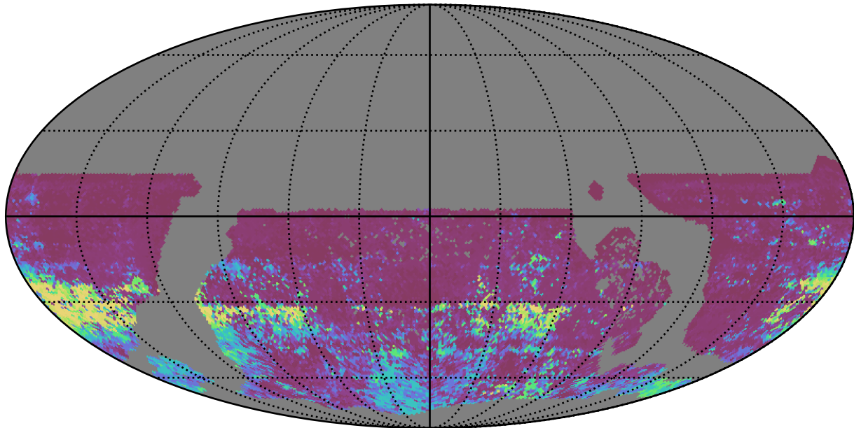
extra_ss_neo4_v3.4_10yrs WFD r band: 75th Percentile Intranight Timespan
