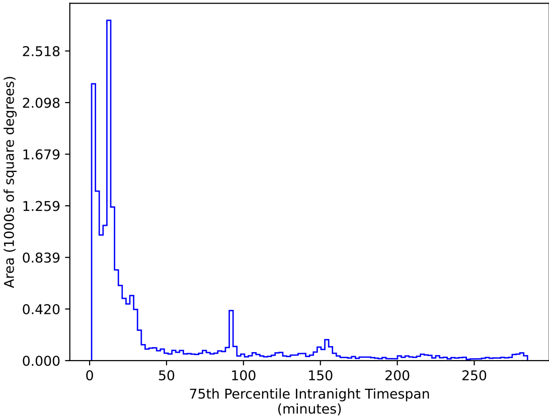
extra_ss_neo4_v3.4_10yrs WFD r band: 75th Percentile Intranight Timespan
