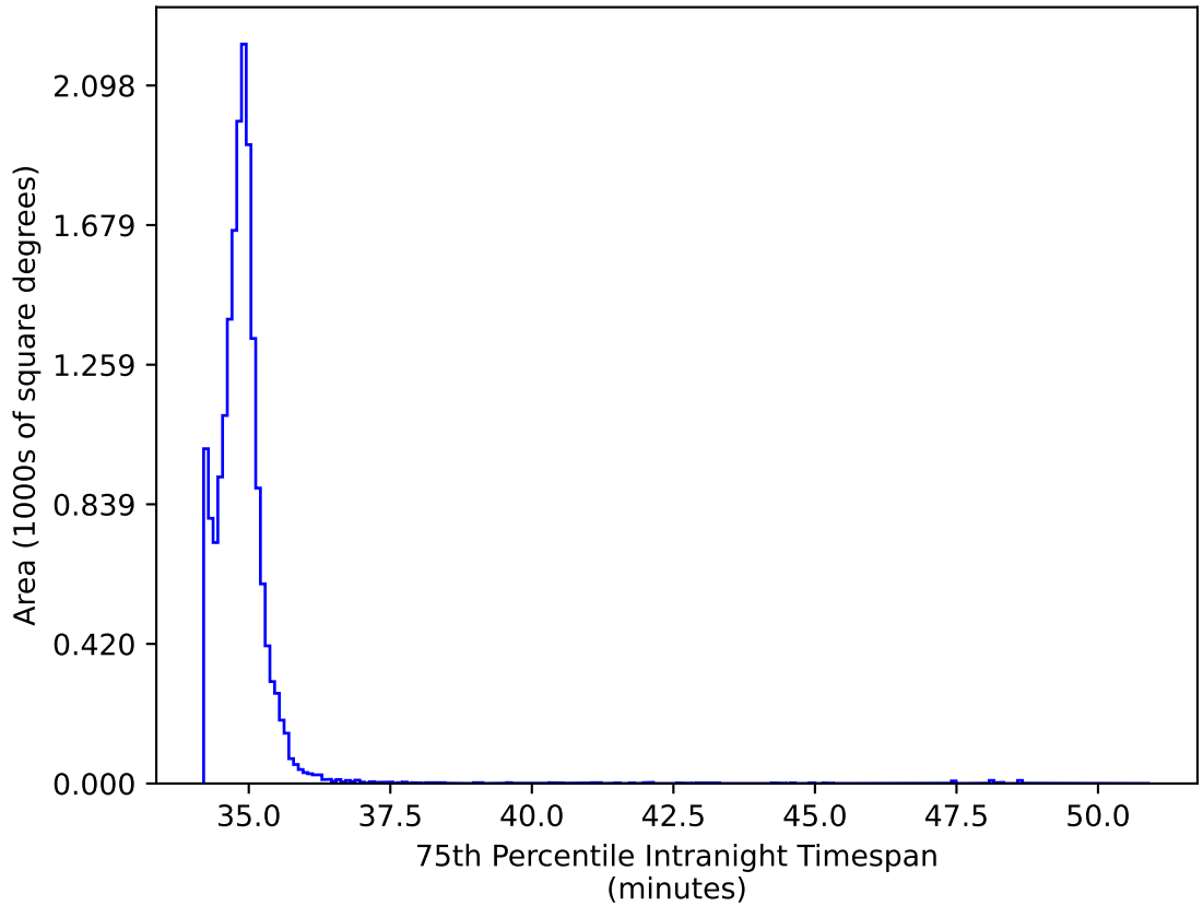
extra_ss_neo4_v3.4_10yrs WFD iz bands: 75th Percentile Intranight Timespan
