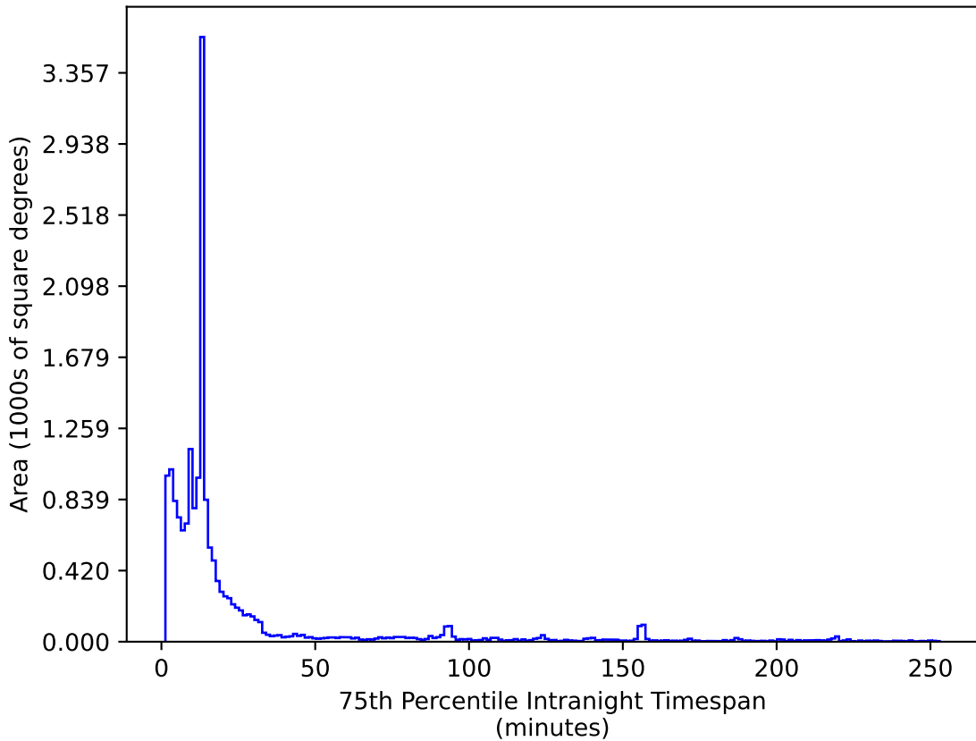
extra_ss_neo4_v3.4_10yrs WFD i band: 75th Percentile Intranight Timespan
