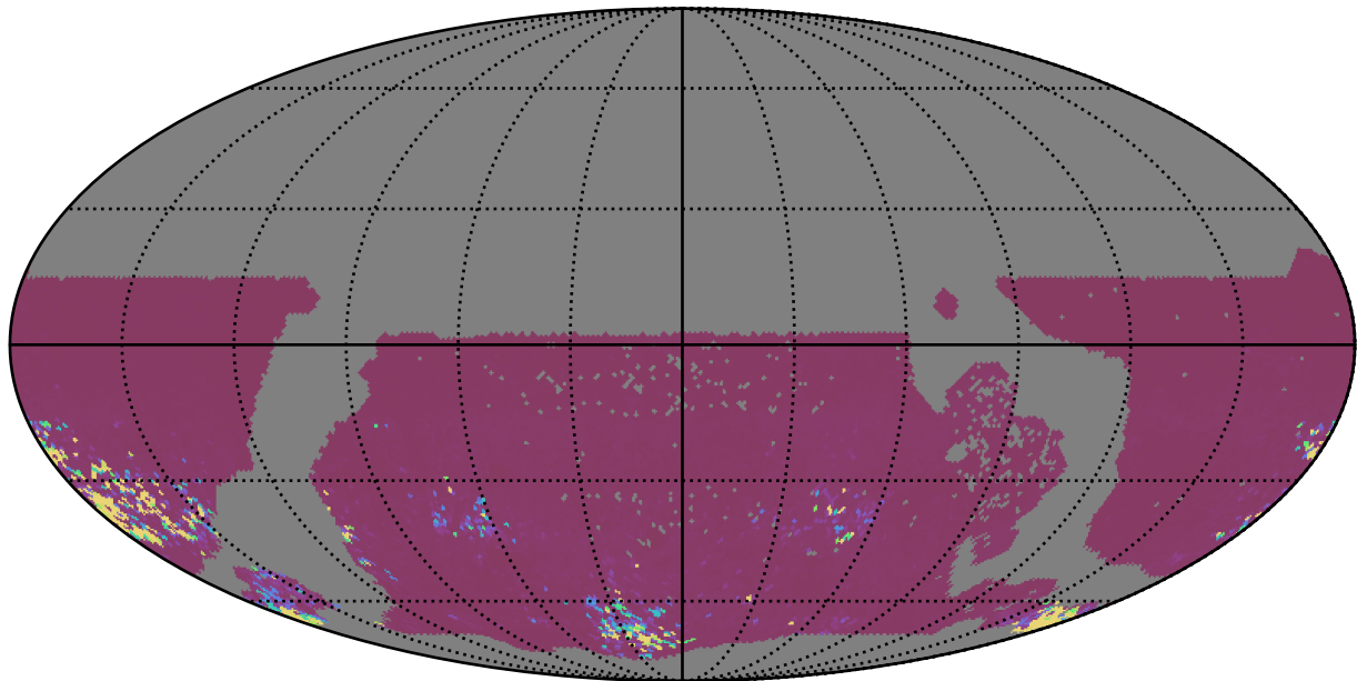
extra_ss_neo4_v3.4_10yrs WFD gr bands: 75th Percentile Intranight Timespan
