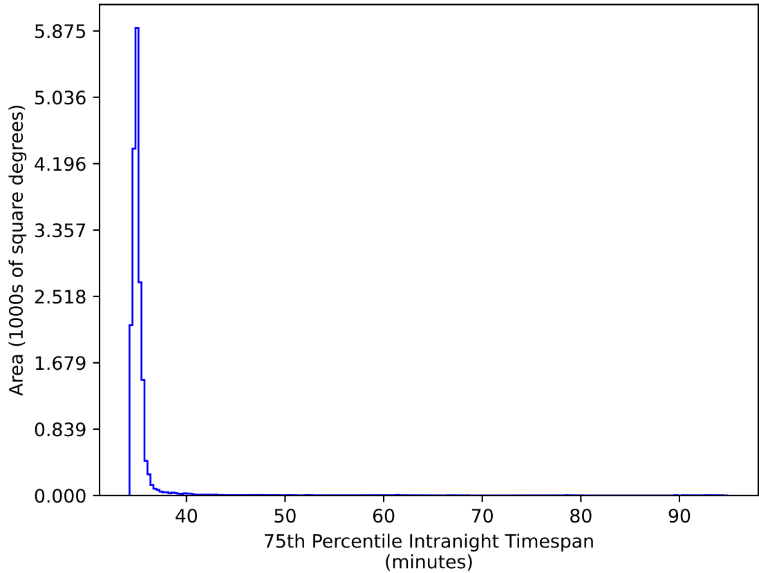
extra_ss_neo4_v3.4_10yrs WFD gr bands: 75th Percentile Intranight Timespan
