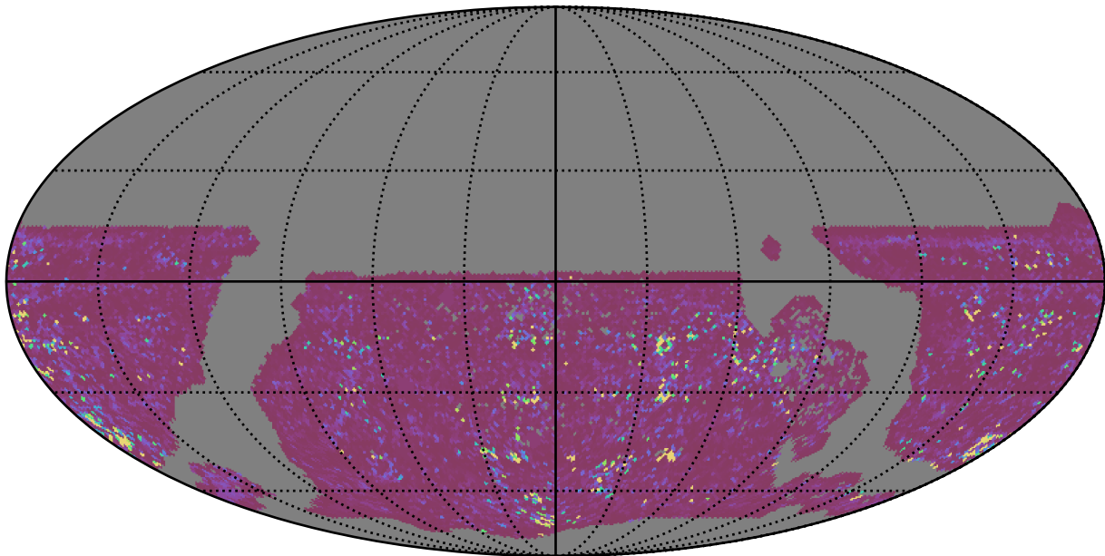
extra_ss_neo4_v3.4_10yrs WFD g band: 75th Percentile Intranight Timespan
