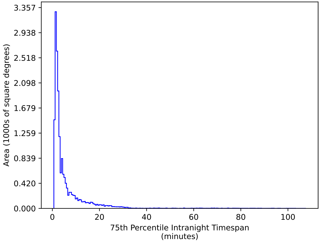
extra_ss_neo4_v3.4_10yrs WFD g band: 75th Percentile Intranight Timespan
