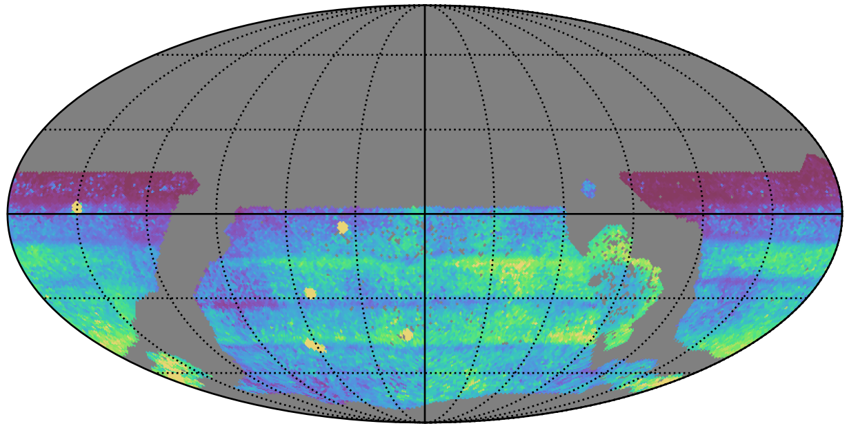
extra_ss_neo4_v3.4_10yrs WFD all bands: 75th Percentile Intranight Timespan
