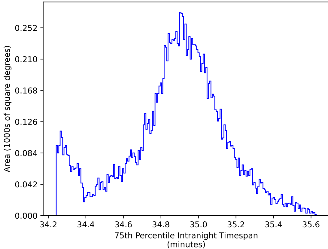
extra_ss_neo4_v3.4_10yrs WFD all bands: 75th Percentile Intranight Timespan
