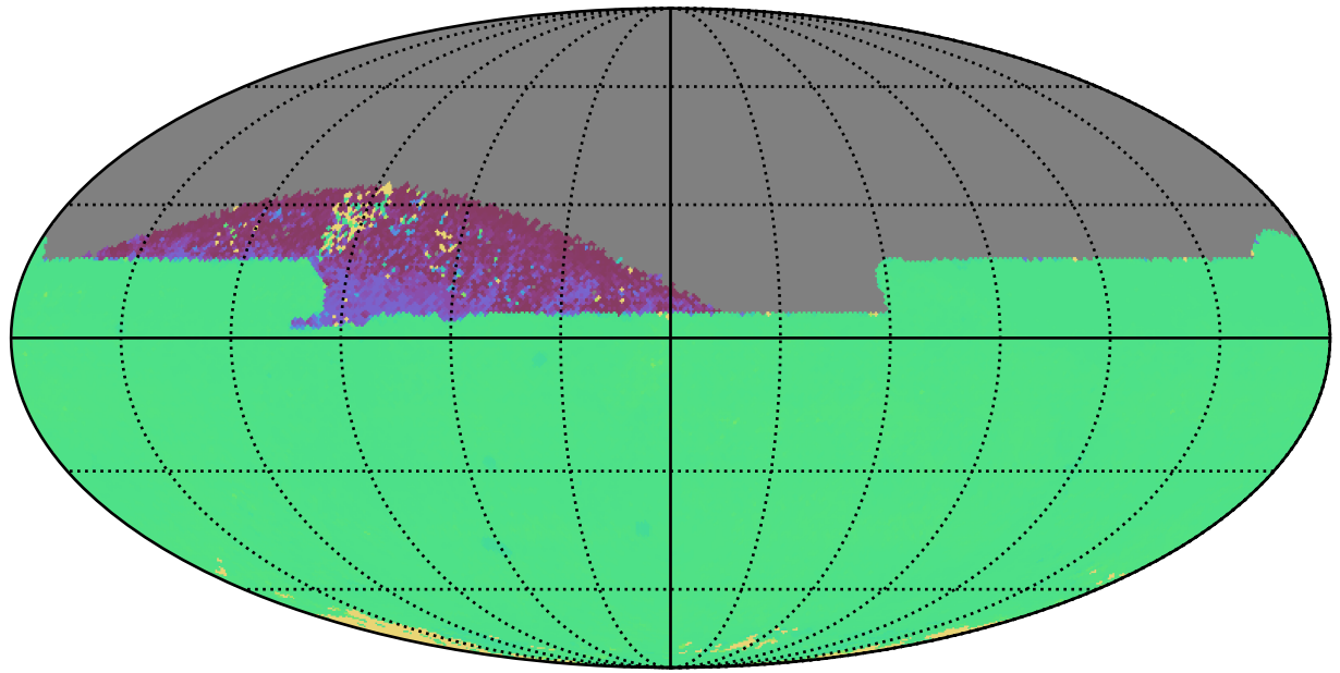
extra_ss_neo4_v3.4_10yrs All sky zy bands: 75th Percentile Intranight Timespan
