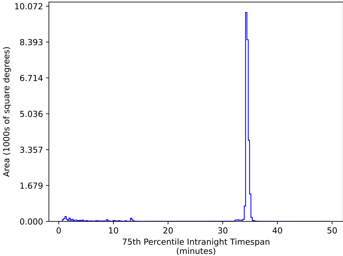
extra_ss_neo4_v3.4_10yrs All sky zy bands: 75th Percentile Intranight Timespan
