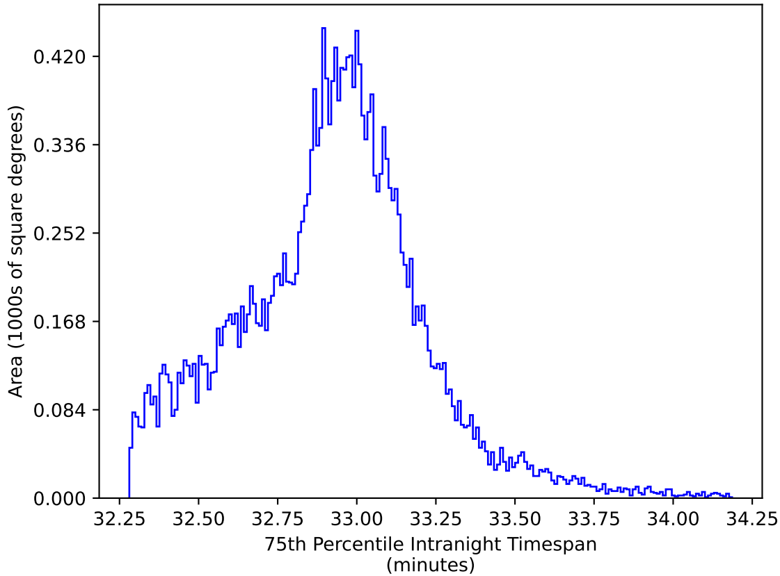
extra_ss_neo4_v3.4_10yrs All sky y band: 75th Percentile Intranight Timespan
