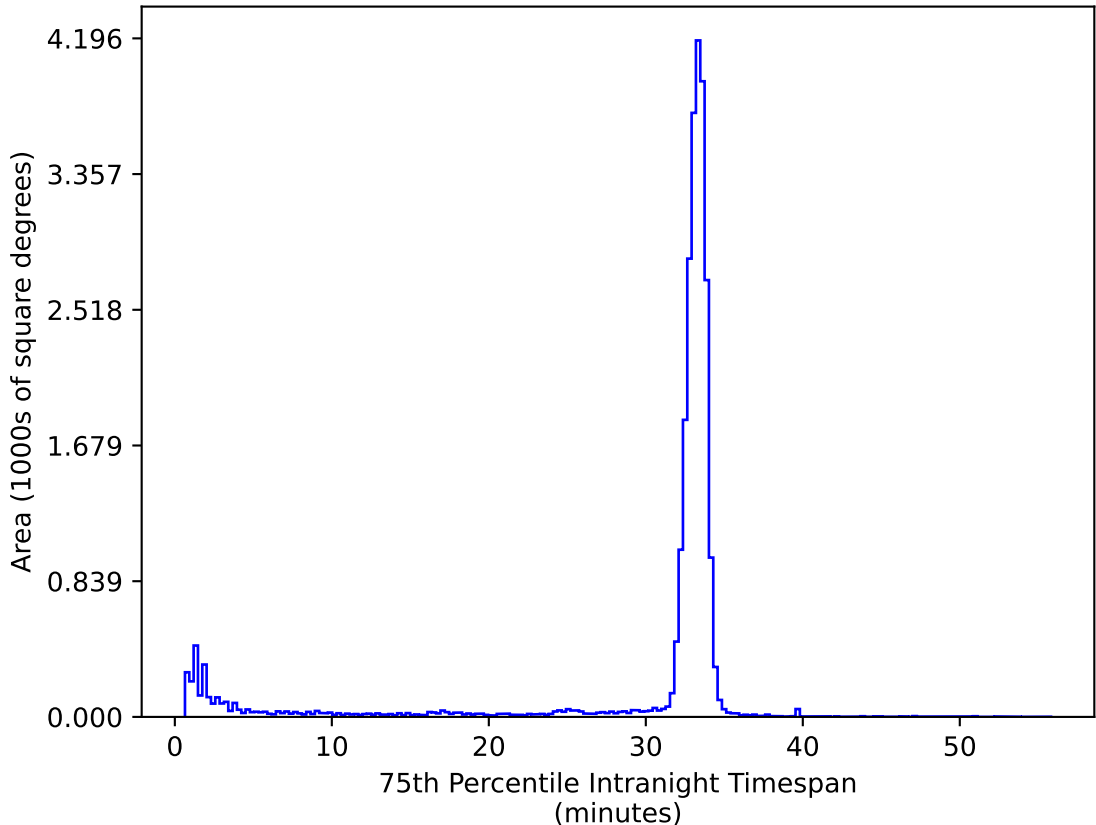
extra_ss_neo4_v3.4_10yrs All sky ug bands: 75th Percentile Intranight Timespan
