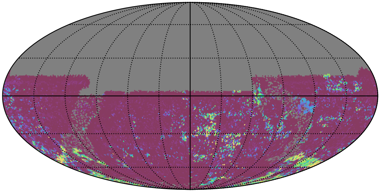
extra_ss_neo4_v3.4_10yrs All sky u band: 75th Percentile Intranight Timespan
