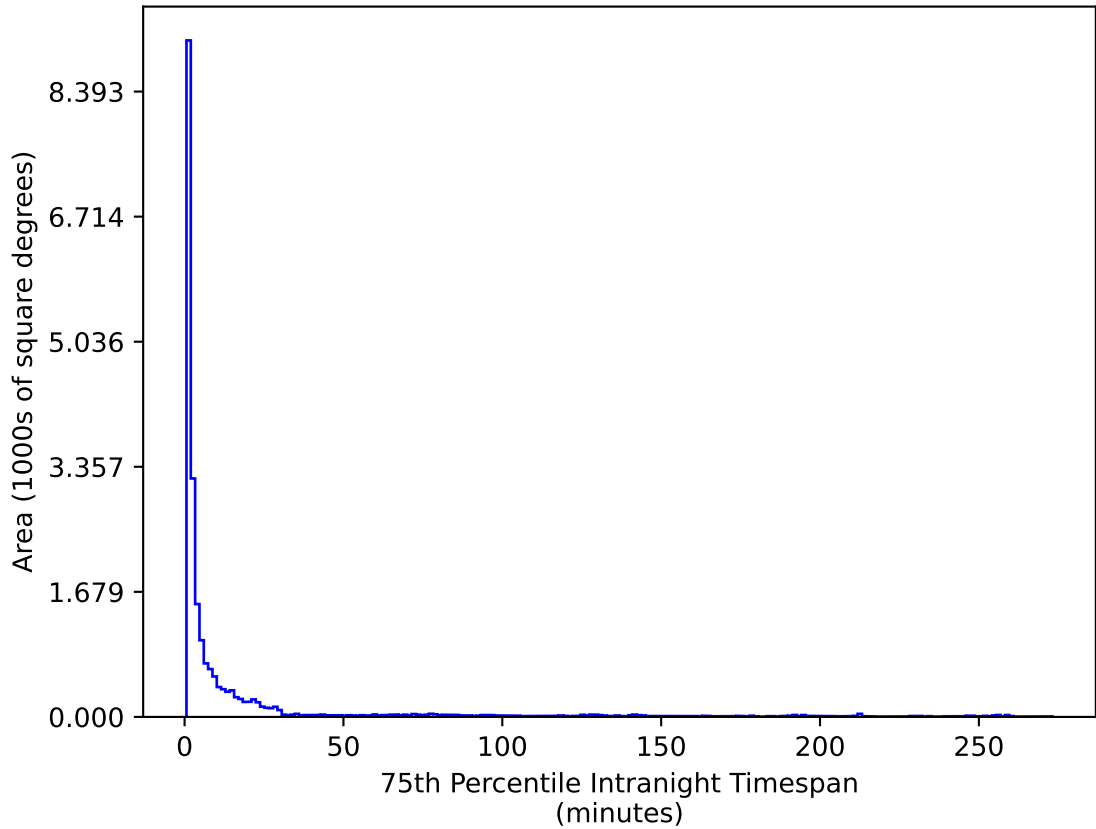
extra_ss_neo4_v3.4_10yrs All sky u band: 75th Percentile Intranight Timespan
