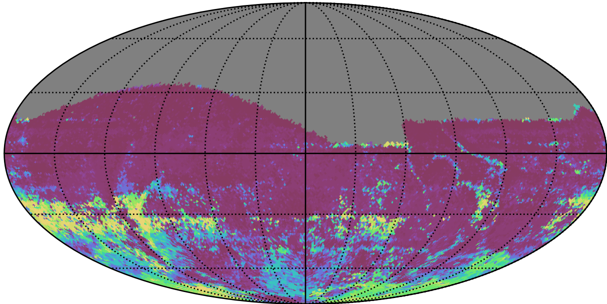
extra_ss_neo4_v3.4_10yrs All sky r band: 75th Percentile Intranight Timespan
