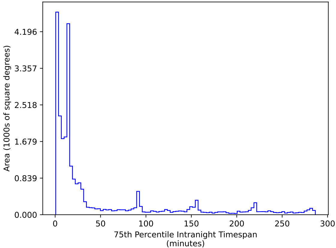
extra_ss_neo4_v3.4_10yrs All sky r band: 75th Percentile Intranight Timespan
