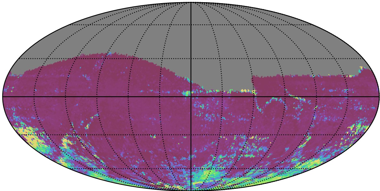
extra_ss_neo4_v3.4_10yrs All sky i band: 75th Percentile Intranight Timespan
