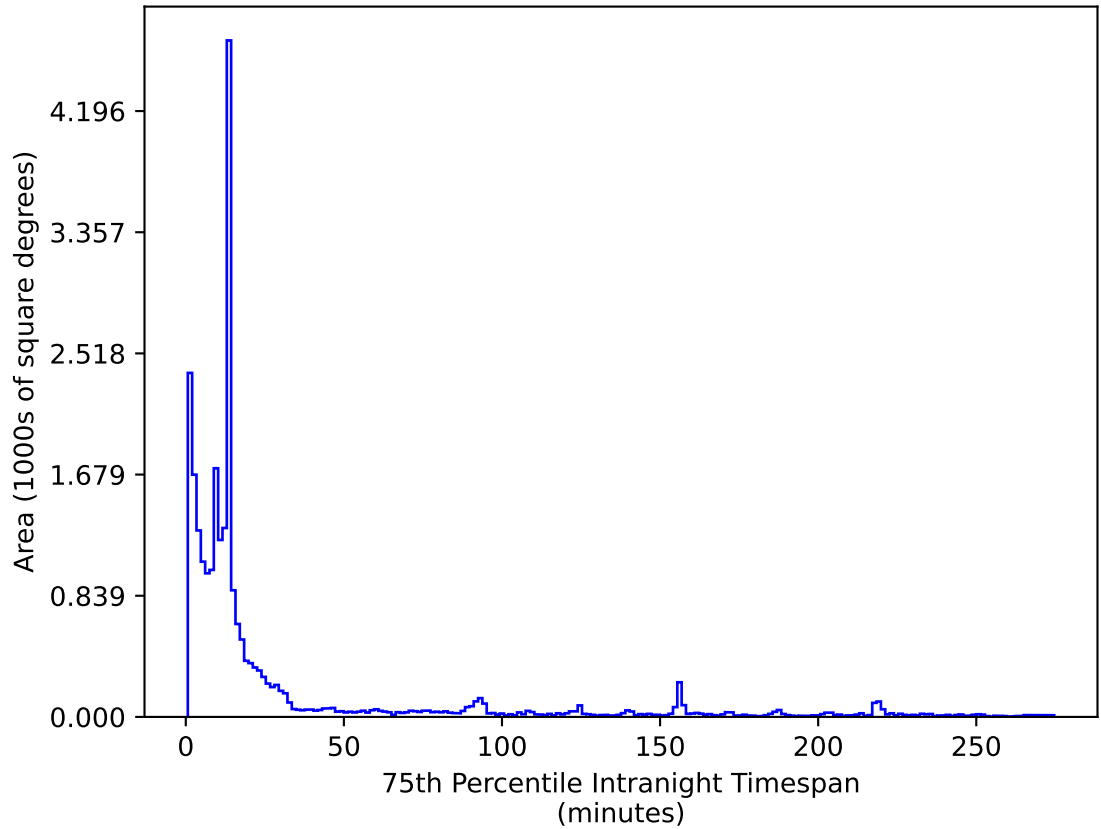
extra_ss_neo4_v3.4_10yrs All sky i band: 75th Percentile Intranight Timespan
