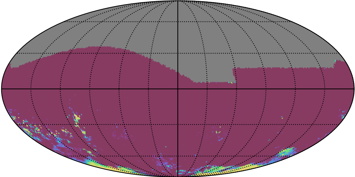
extra_ss_neo4_v3.4_10yrs All sky gr bands: 75th Percentile Intranight Timespan
