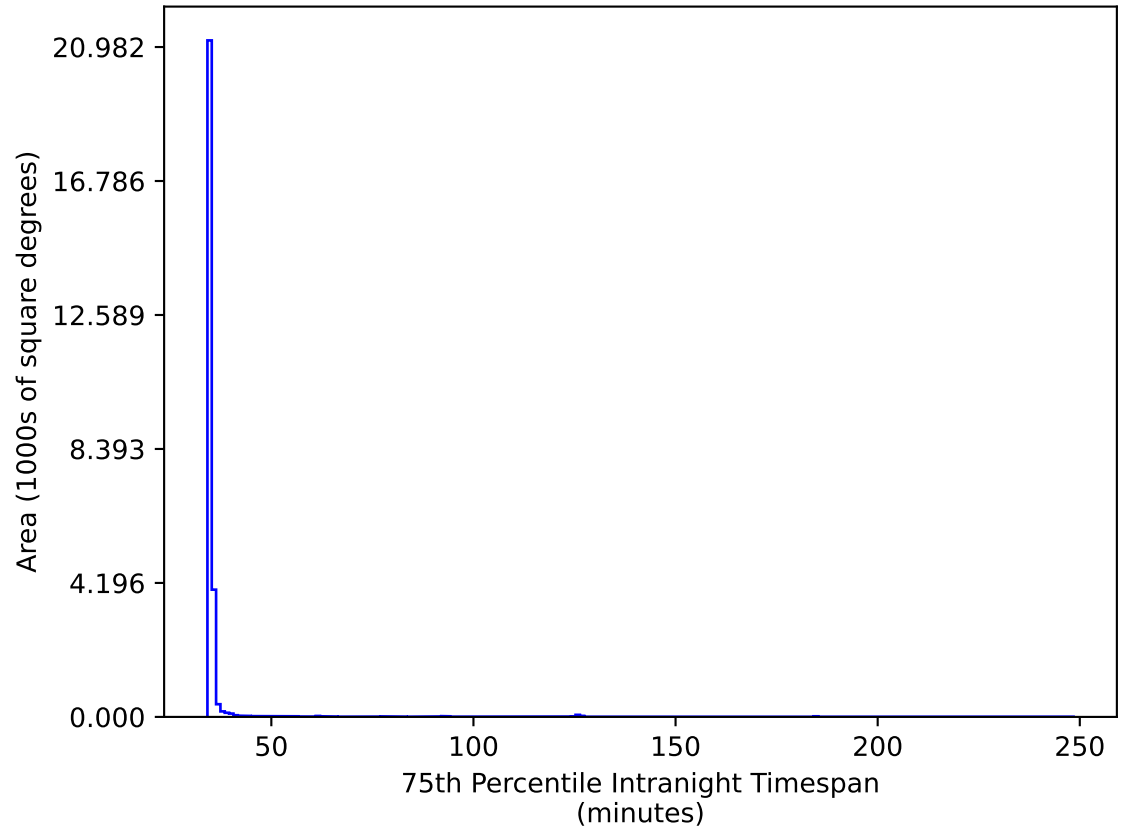
extra_ss_neo4_v3.4_10yrs All sky gr bands: 75th Percentile Intranight Timespan
