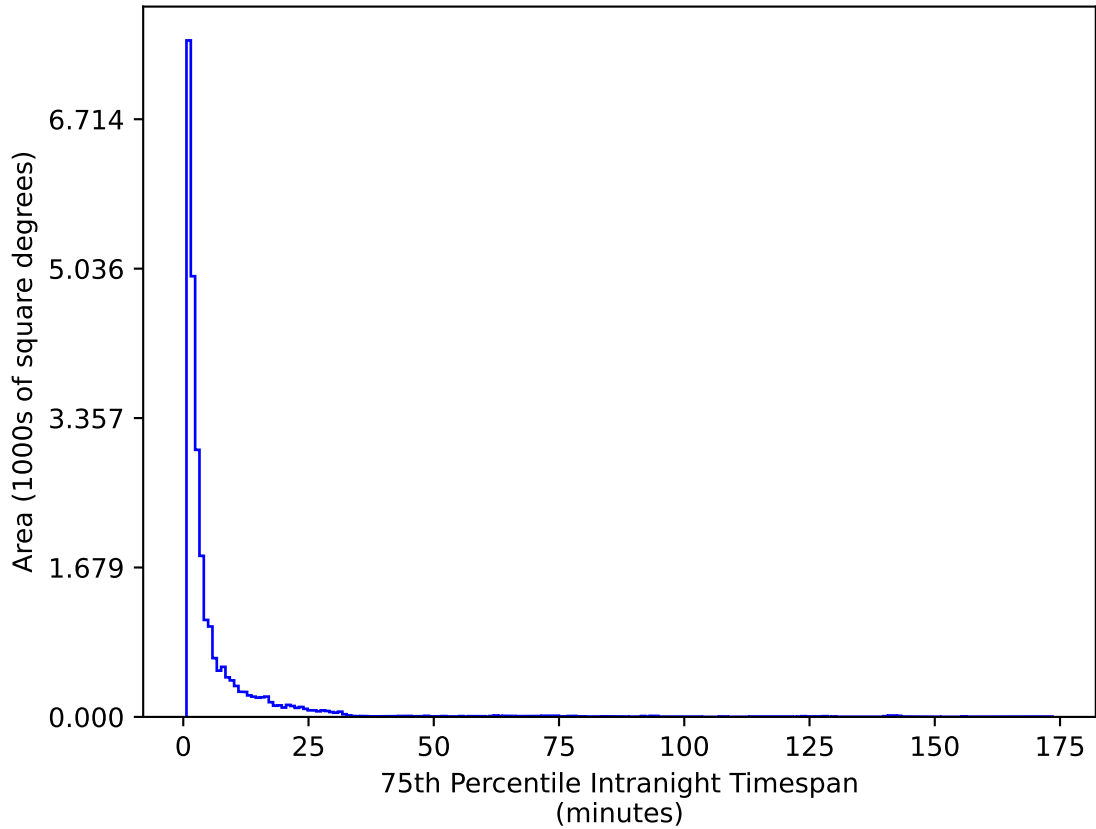
extra_ss_neo4_v3.4_10yrs All sky g band: 75th Percentile Intranight Timespan
